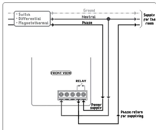
Standard Connecting Diagram:
