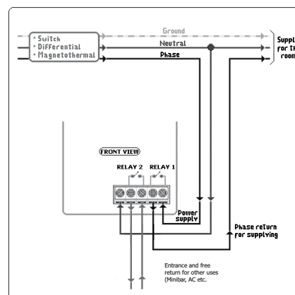
Intelligent Magnetic Stripe and RFID Connecting Diagram:
